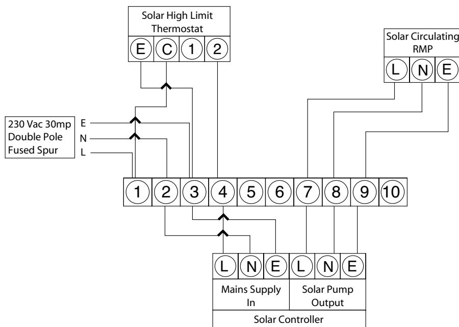
Fig1: Isolation of Input: Closure of Two Port Valve & Disconnection Pump
