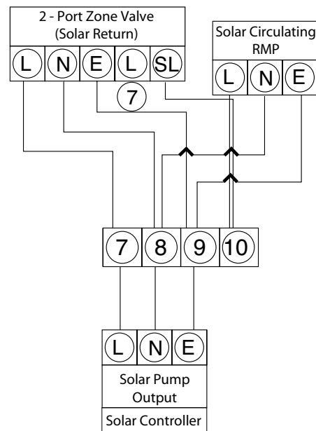
Fig2: Alternative arrangement for Solar Pump stations without integral gravity break check valve
