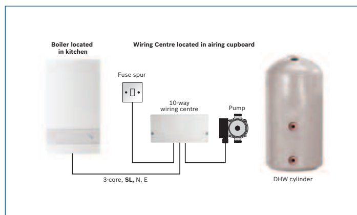
Existing boiler system layout
