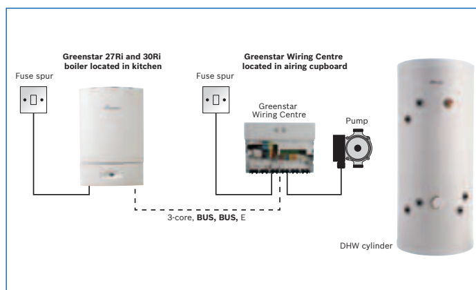
System layout with a Greenstar Wiring Centre
