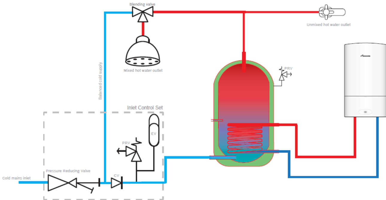
Fig. 1: Example use of balanced cold connection
