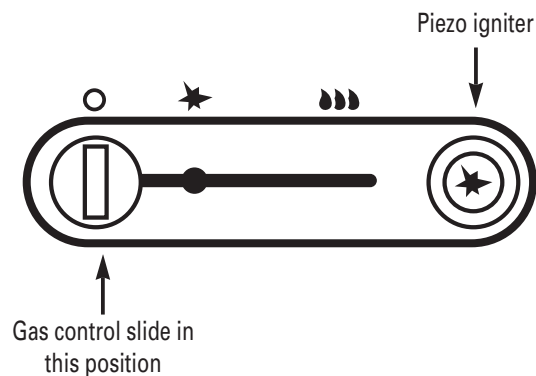
Fig. 5. Gas control slide – shut down position
