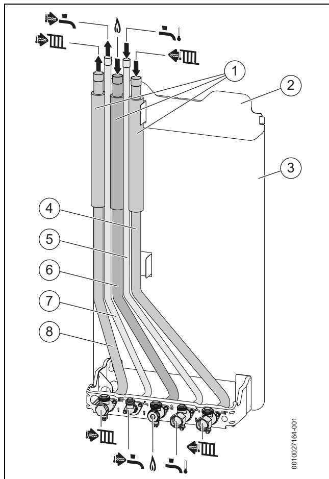
Fig. 1 Vertical pre-piping assembly
